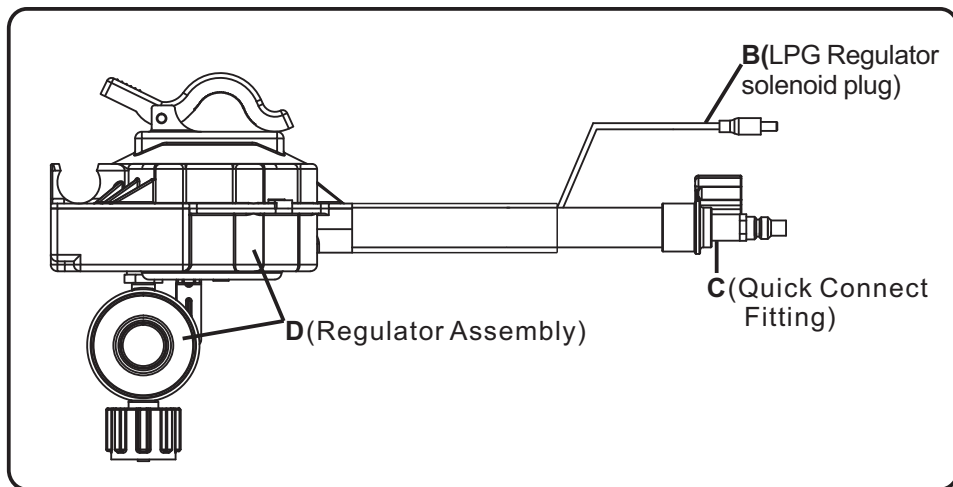
A(LPG Regulator/Hose Assembly)
