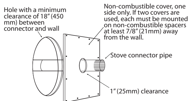
Figure 7 ONLY APPROVED CANADIAN WALL PASS THROUGH
