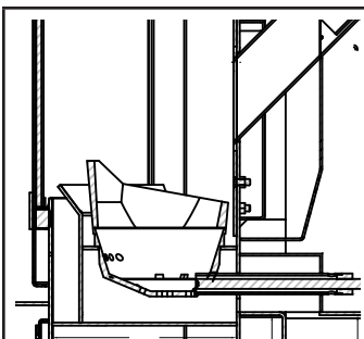
Figure 4 Pot de combustion PSBF66W
