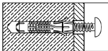
Solid wall
