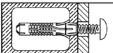
Hollow wall
