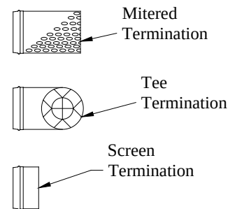
Fig 17. (Horizontal Terminations)
