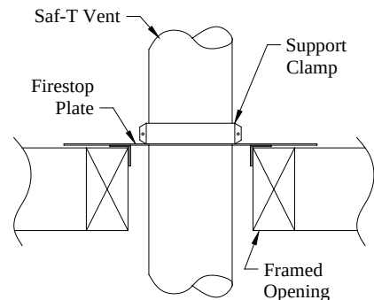
Fig 10. (Fire Stop)
