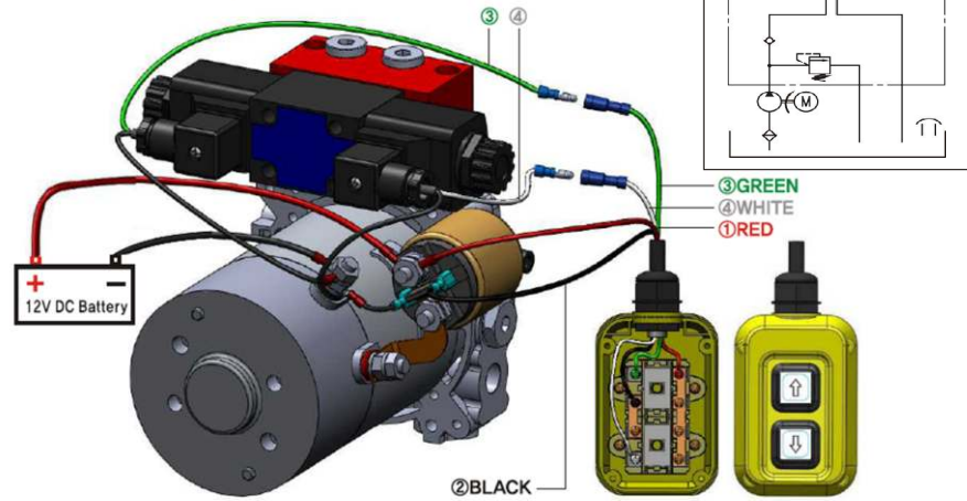
Unidirectional Motor
