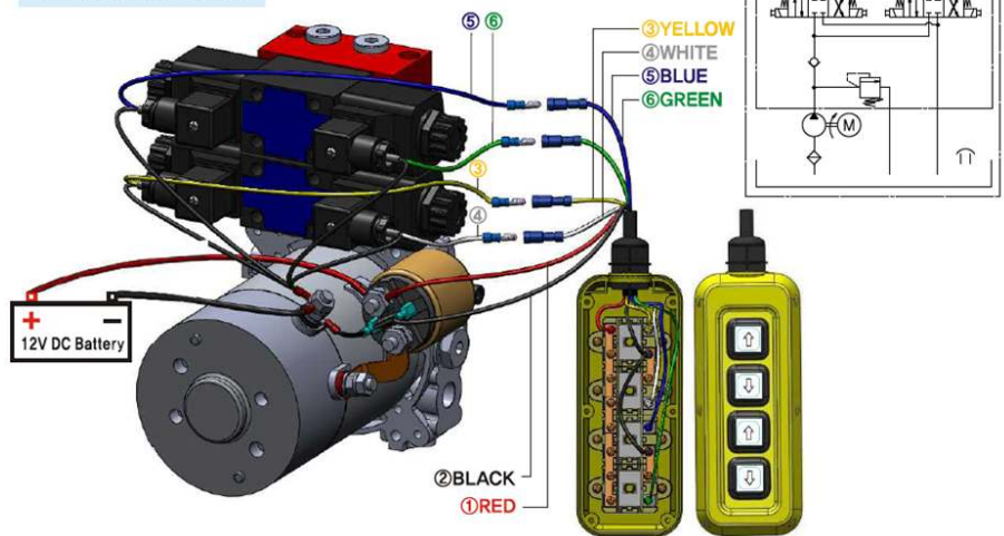
Unidirectional Motor
