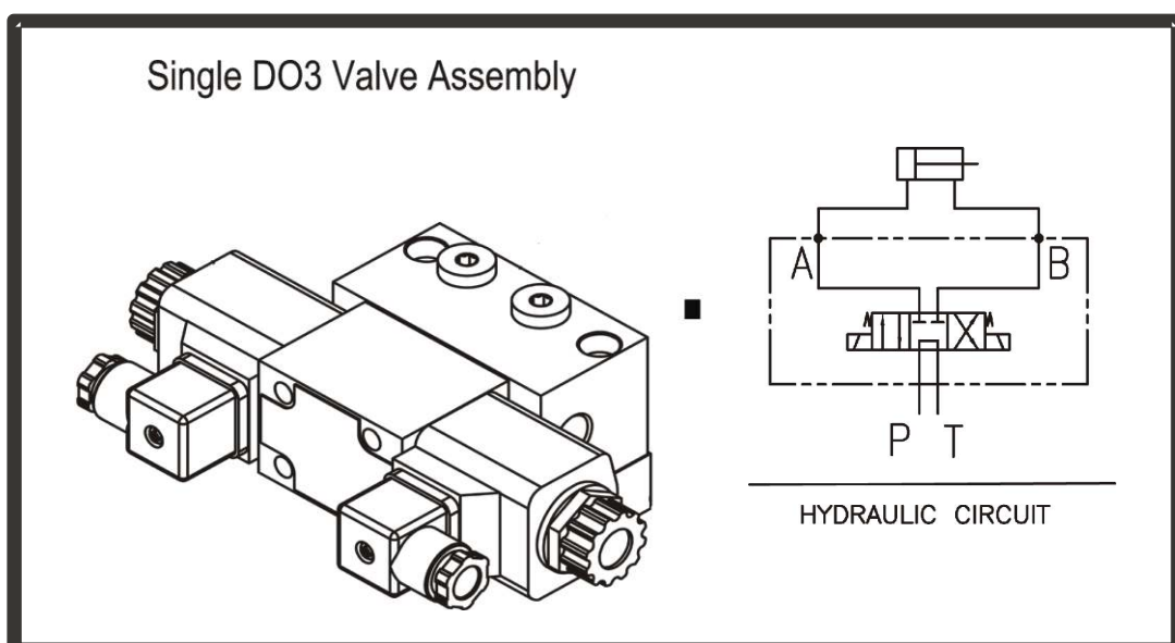
Schematic 1
