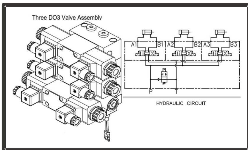
Schematic 3
