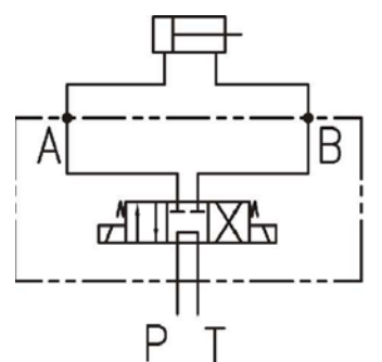
CIRCUIT HYDRAULIQUE
