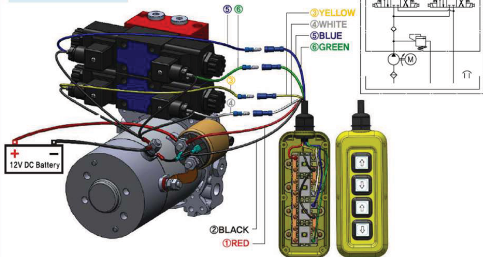
Unidirectional Motor
