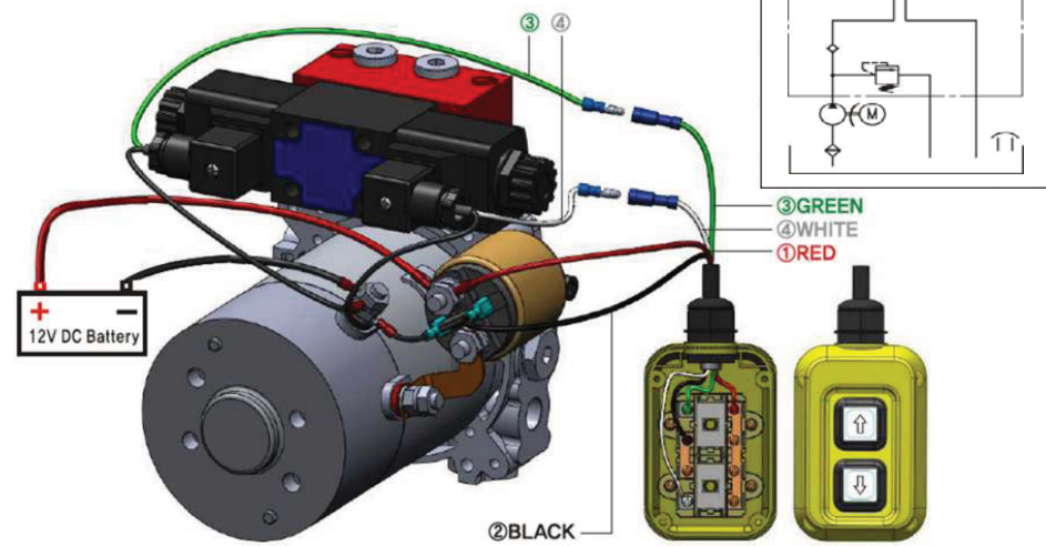
Unidirectional Motor
