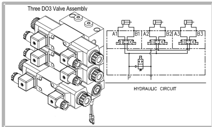
Schematic 3
