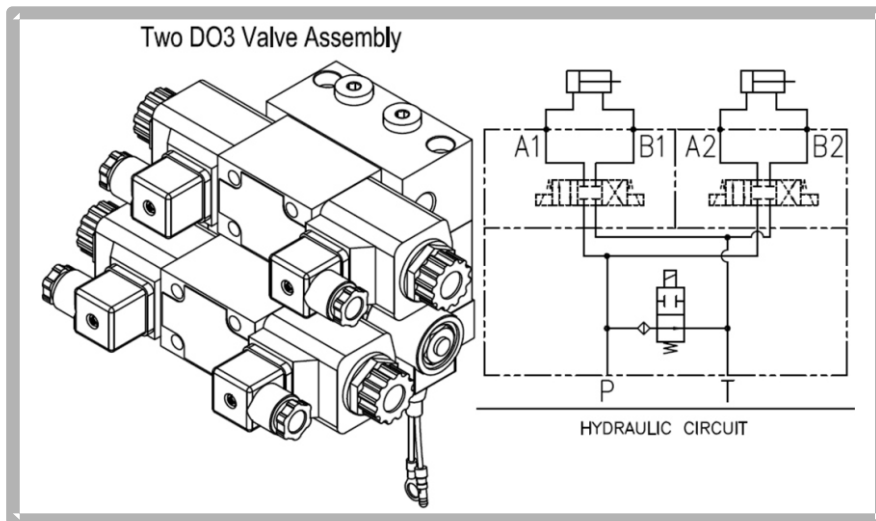
Schematic 2
