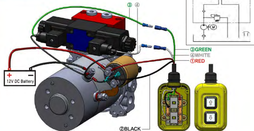
Unidirectional Motor
