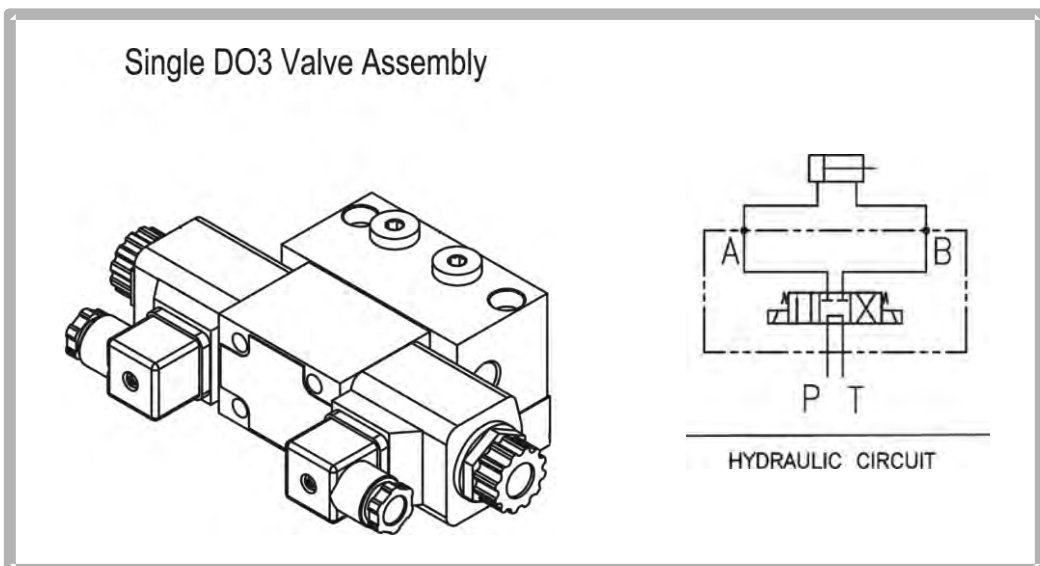
Schematic 1
