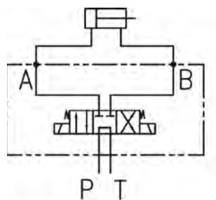
CIRCUIT HYDRAULIQUE
