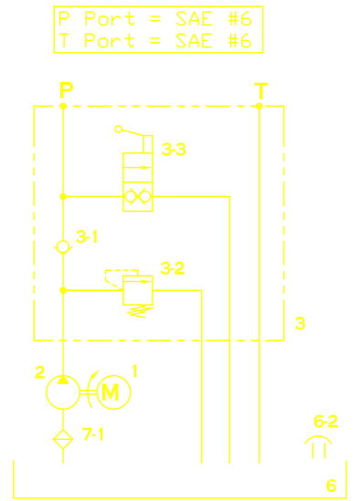
HYDRAULIC CIRCUIT
